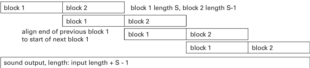
Figure 7.4 Convolution input and output block sizes and the overlap-add operation.
