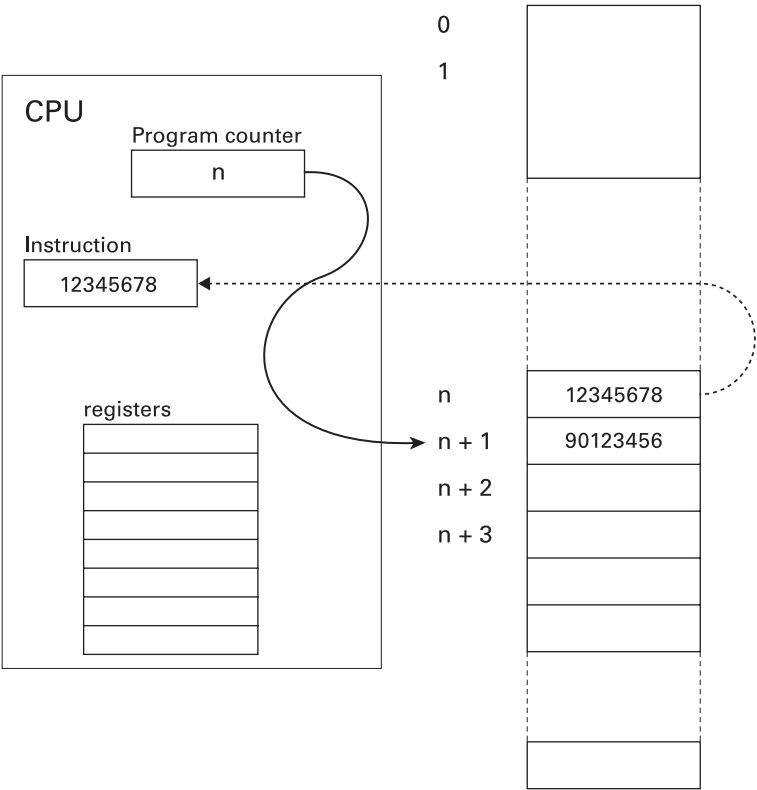
Figure F.4 CPU with registers.
