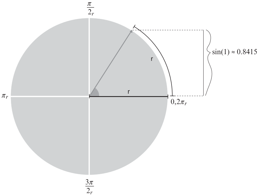
Figure 2.12 The radian.
