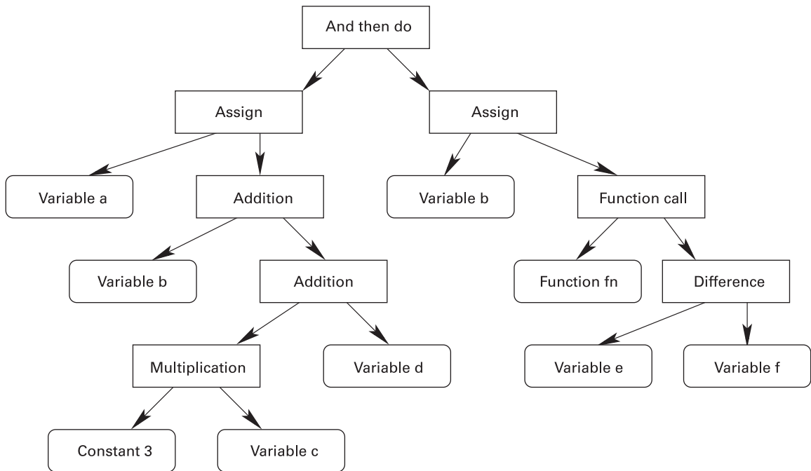
Figure F.7 Parse tree.
