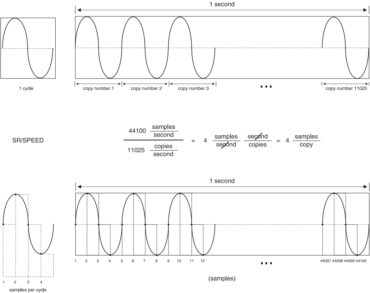
Figure 4.2 Copying a waveform.
