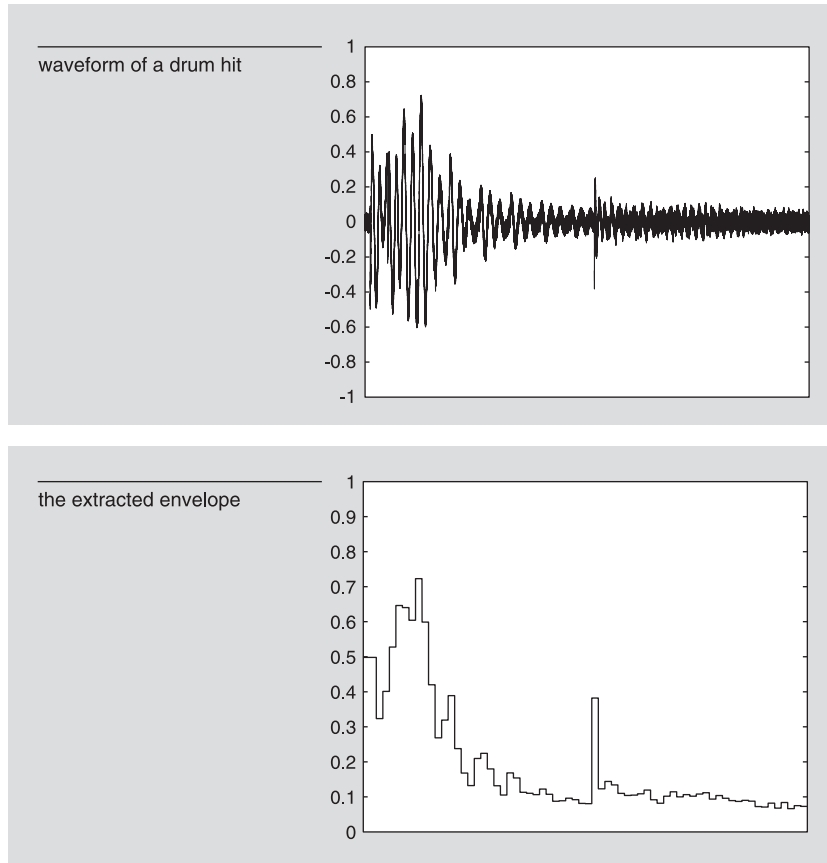
Figure 2.7 Extracting an amplitude envelope.
