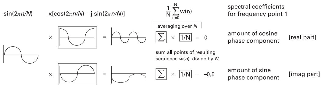
Figure 7.1 The DFT operation on frequency point 1, showing how a complex sinusoid is used to detect the sine and cosine phase components of a signal.
