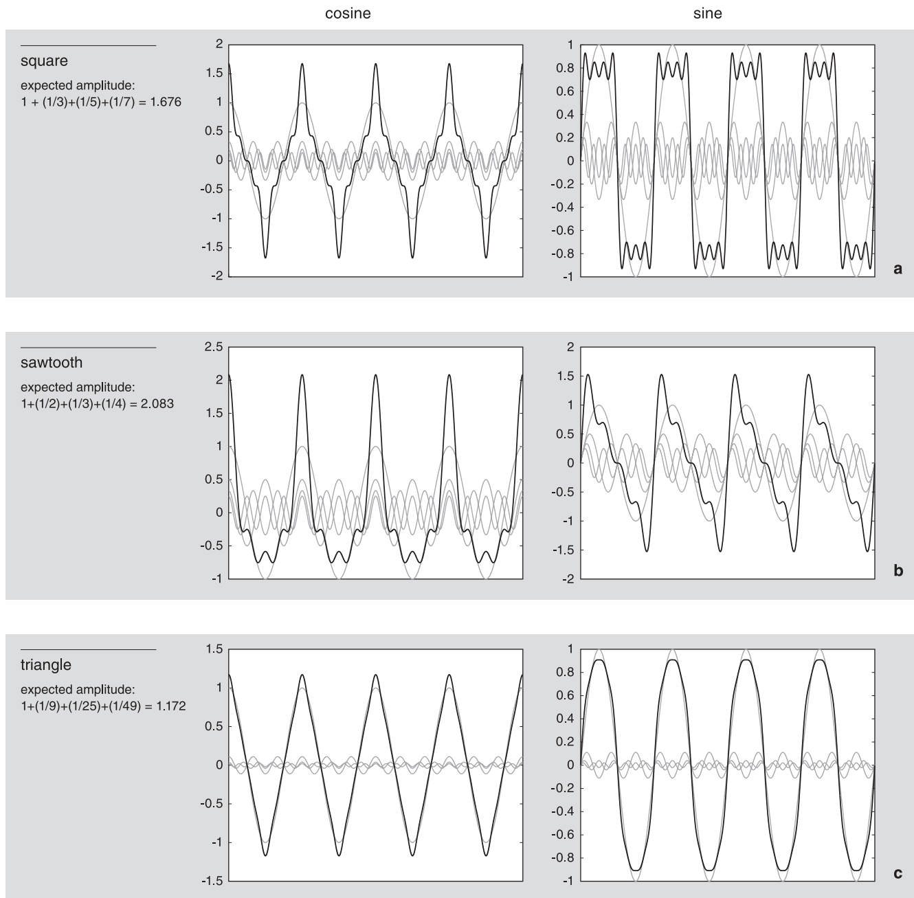
Figure 2.16 Additive waveform generation using sines or cosines.
