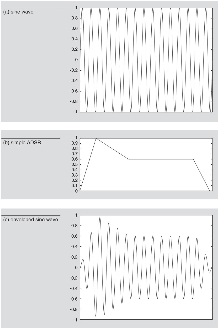
Figure 2.6 Enveloping an audio signal.
