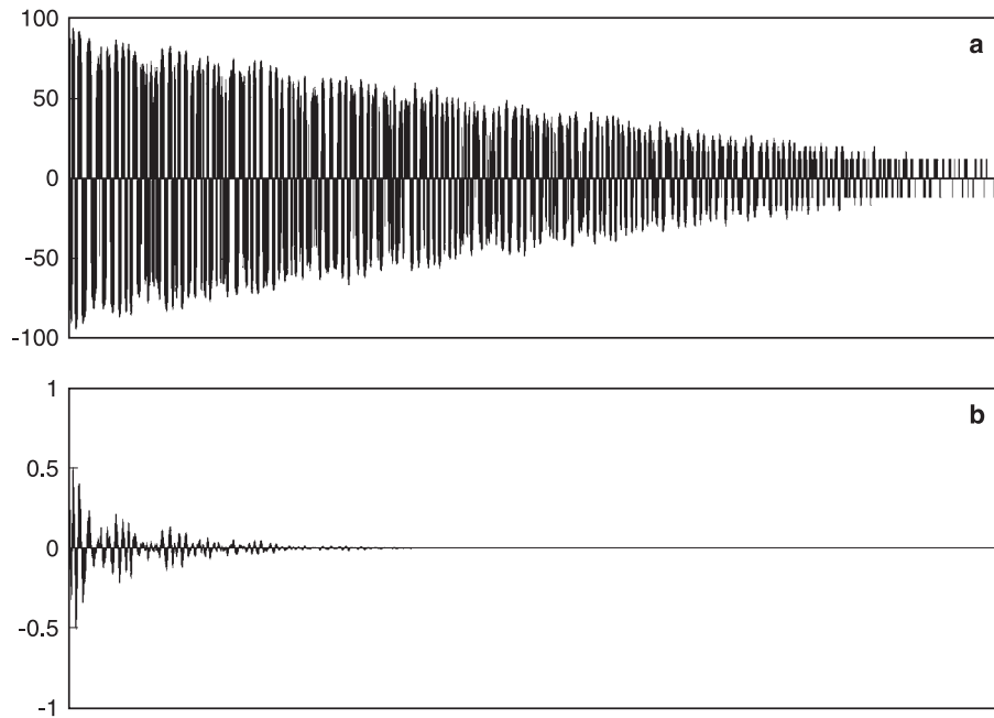
Figure 2.2 Reverb decay on (a) dB and (b) amplitude vertical scales.
