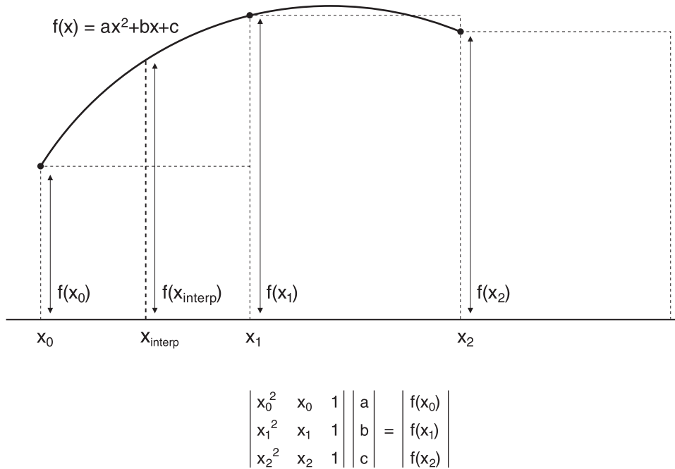
Figure 4.5 Quadratic interpolation.
