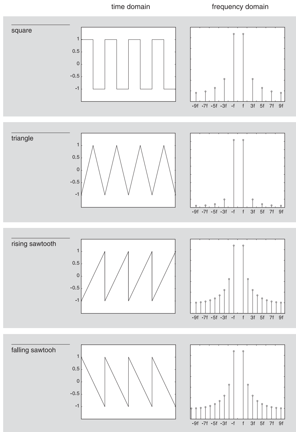
Figure 2.13 Standard geometric waveforms.
