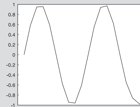
Figure 2.19 Comparison of truncated and interpolated lookup.
